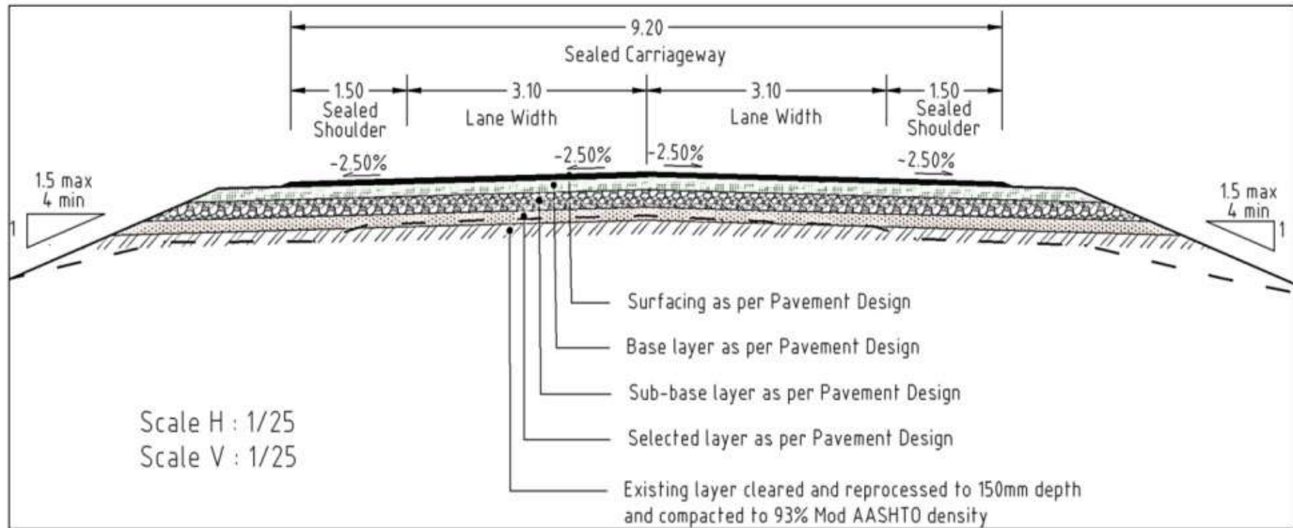
Figure 2-10: Typical Road Cross Section
